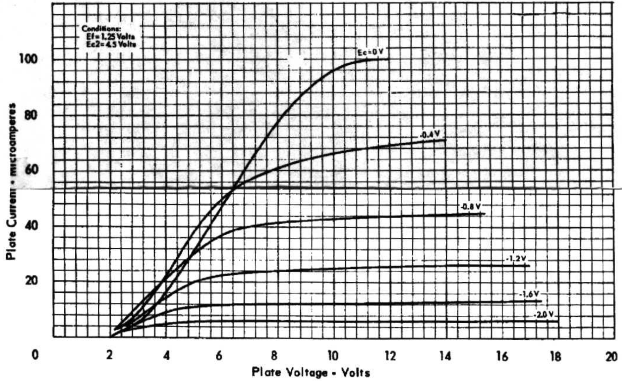
AVERAGE PLATE CHARACTERISTICS
