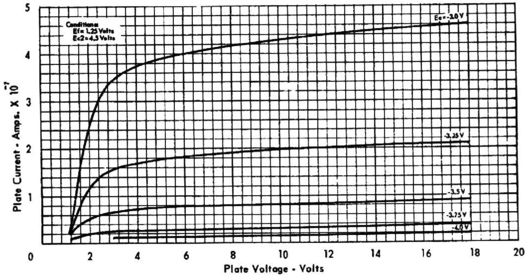
AVERAGE PLATE CHARACTERISTICS
