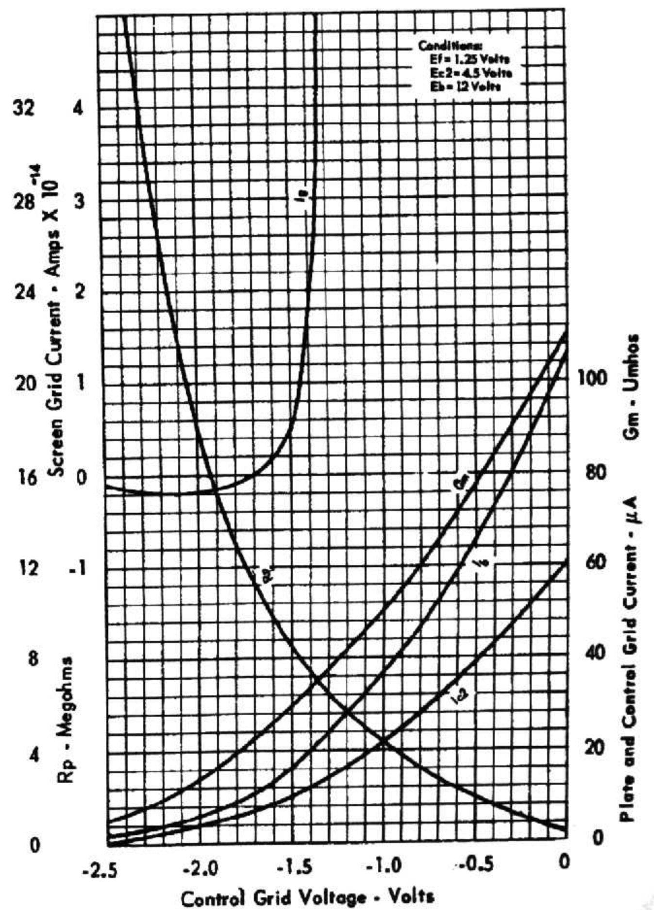
AVERAGE TRANSFER CHARACTERISTICS
