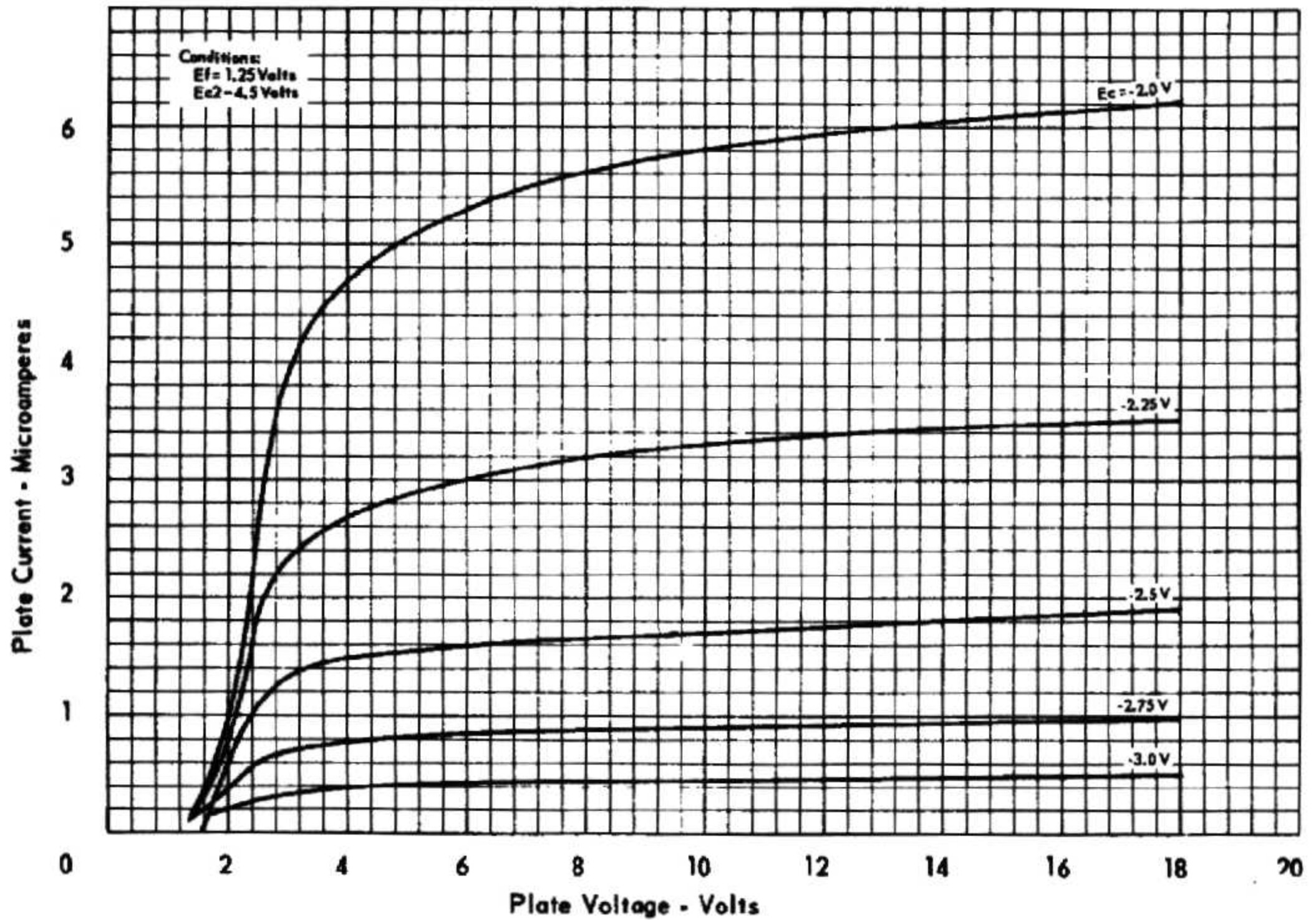
AVERAGE PLATE CHARACTERISTICS
