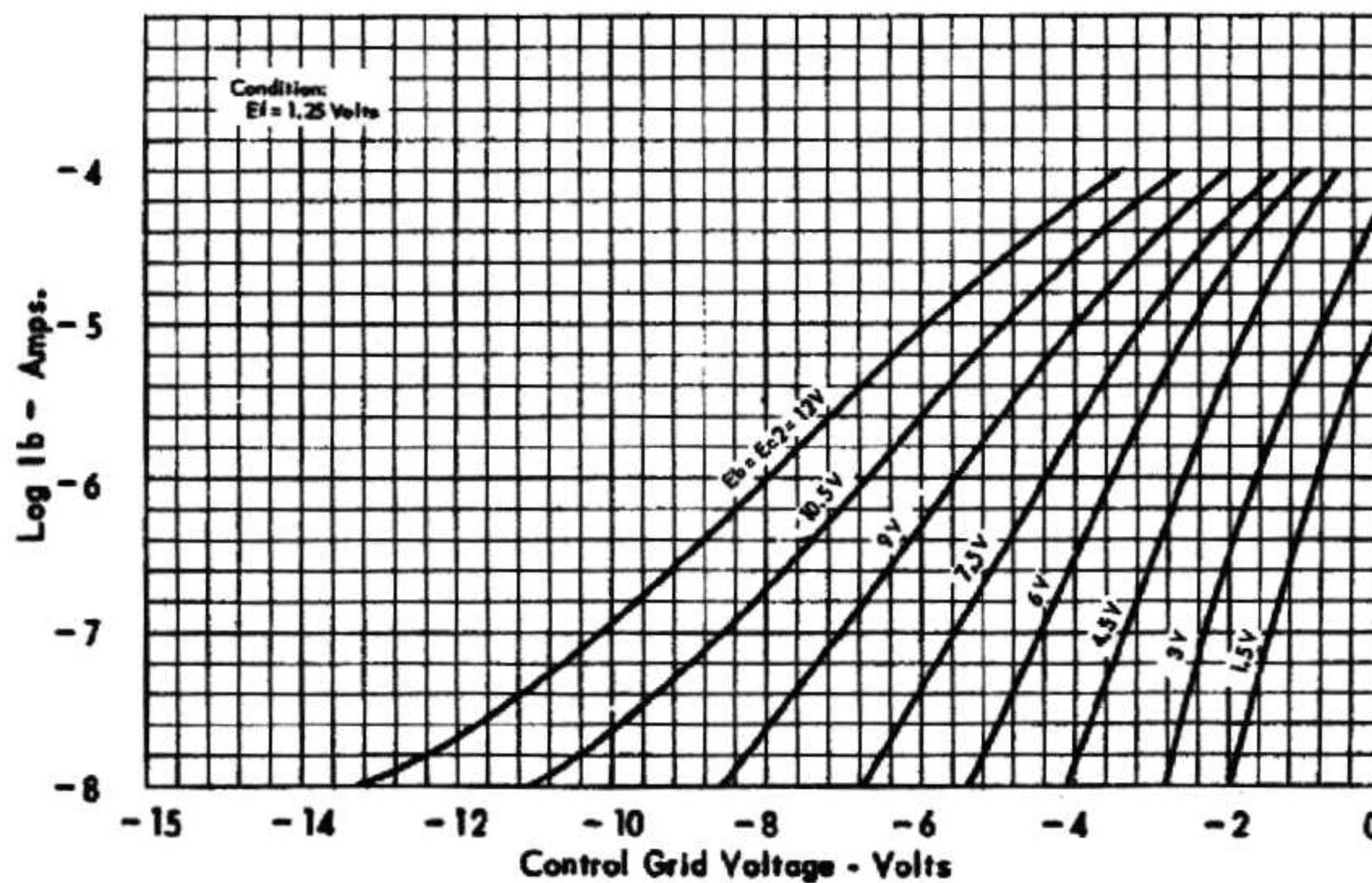
AVERAGE TRANSFER CHARACTERISTICS
